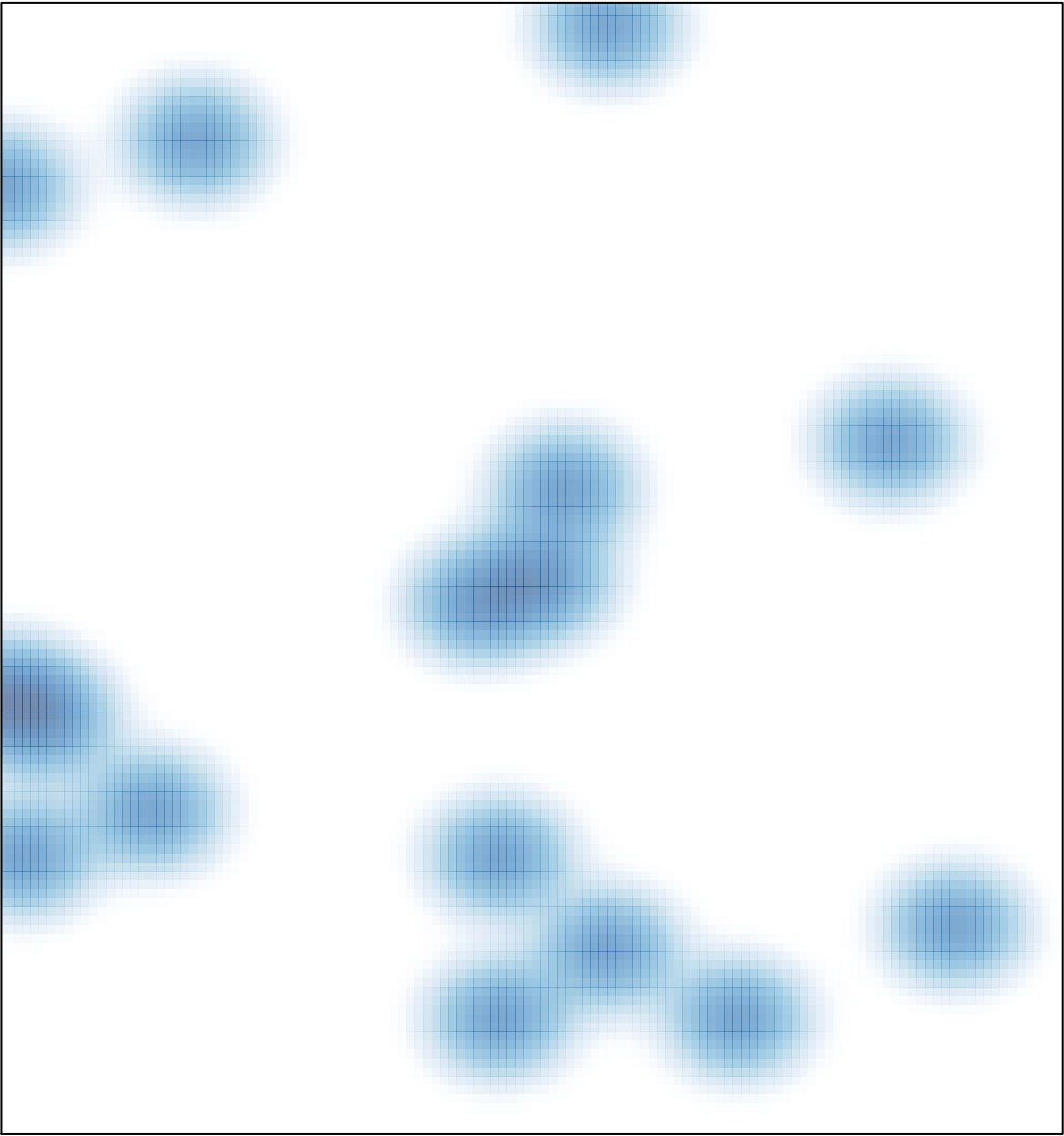
# features = 18 , max = 1
